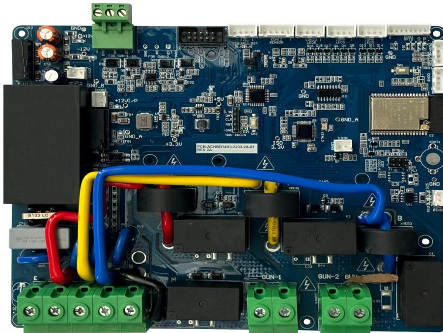
Figure 2 AC Hybrid Charger Controller
