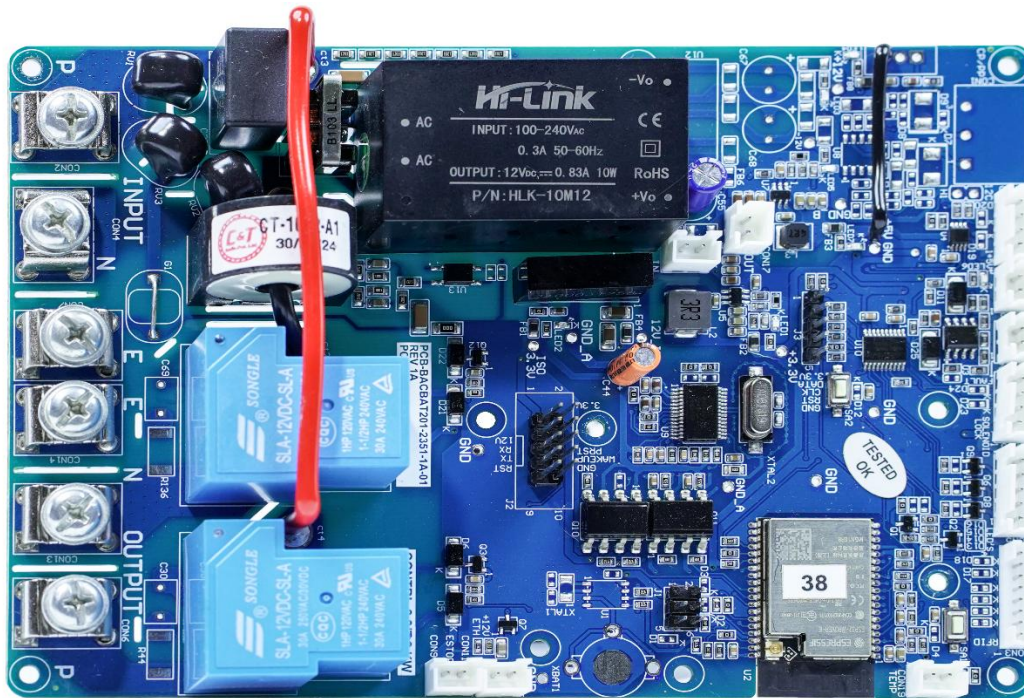
Figure 2 Bharat AC Single Socket Charger Controller with RFID
